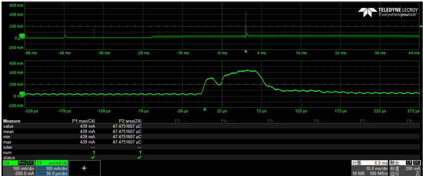
Max Impulse Current When Powered On
