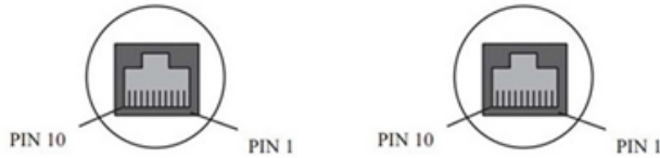
CD220(E) Data Port Pinout:
